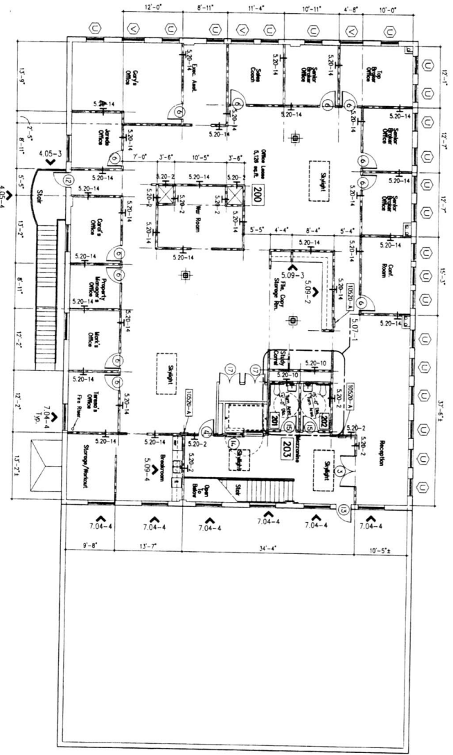
5.01-1 FLOORPLAN - LEVEL 2 1/8"=1'-0"
